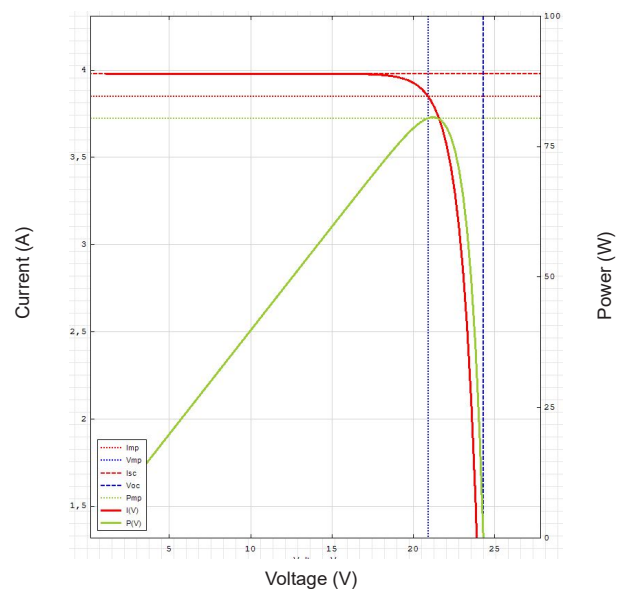
RNG-80D-SS Characteristics Versus Voltage
